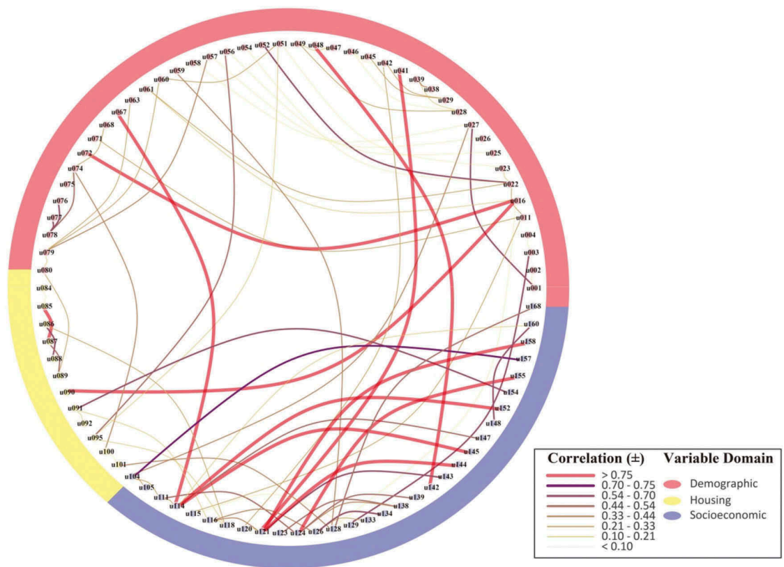
Figure 4. Minimum spanning tree (presented in circle layout) of the census variables after the PCA-based filter. The thickness of curve indicates the absolute value of the person correlation coefficient. The value that above \pm 0.75 is highlighted by red thicker line, which therefore will be removed in the next phases.
